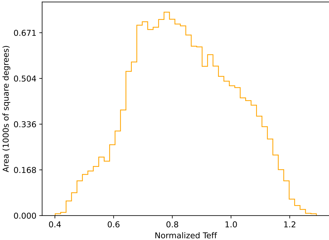
too_elab_r256_d3_ugrizy_v3.4_10yrs WFD r band: Normalized Teff
