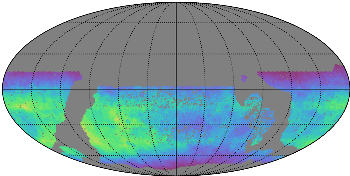
too_elab_r256_d3_ugrizy_v3.4_10yrs WFD i band: Normalized Teff
