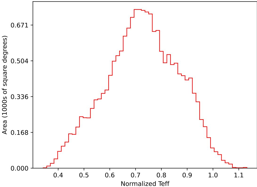
too_elab_r256_d3_ugrizy_v3.4_10yrs WFD i band: Normalized Teff
