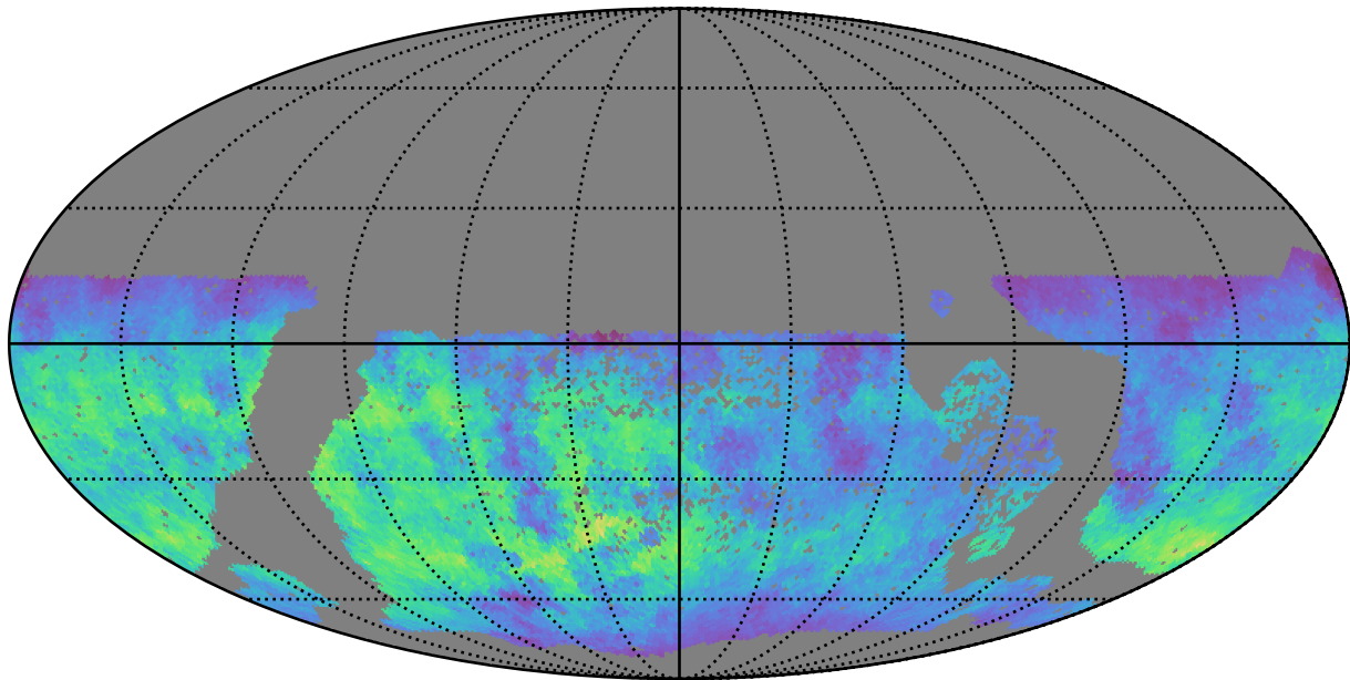
too_elab_r256_d3_ugrizy_v3.4_10yrs WFD g band: Normalized Teff
