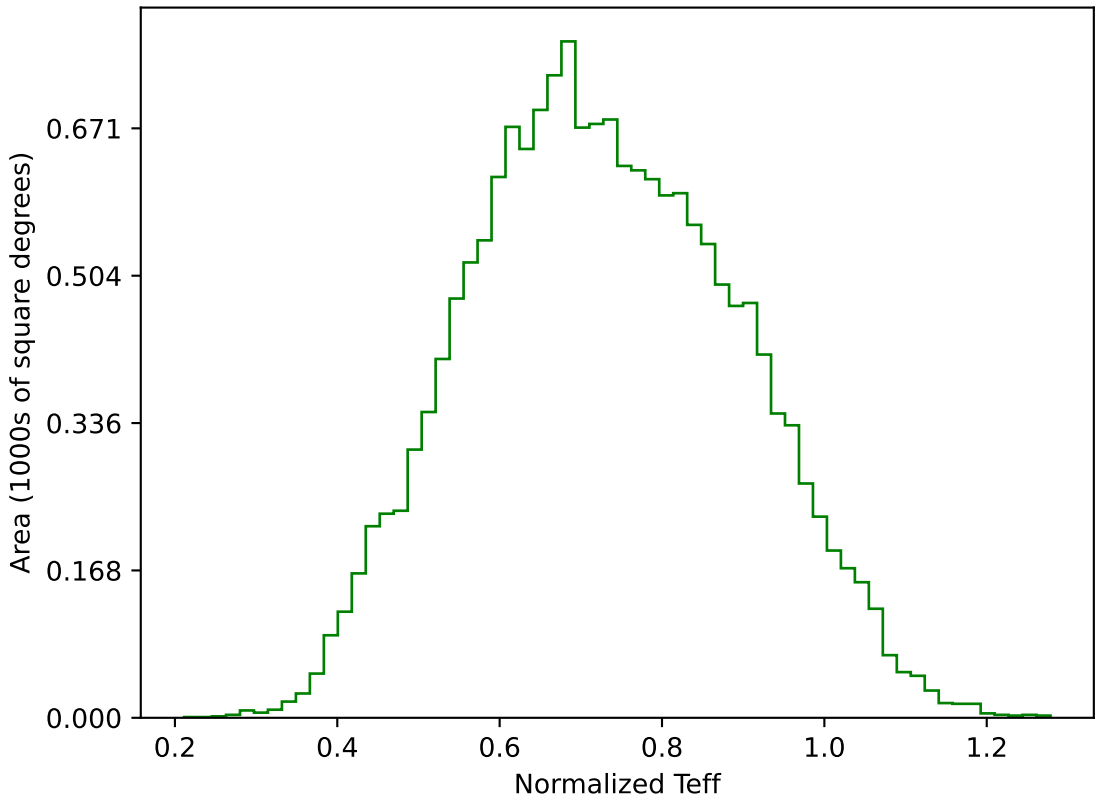
too_elab_r256_d3_ugrizy_v3.4_10yrs WFD g band: Normalized Teff
