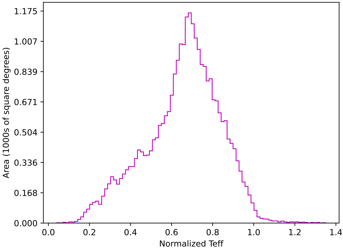
too_elab_r256_d3_ugrizy_v3.4_10yrs All sky z band: Normalized Teff
