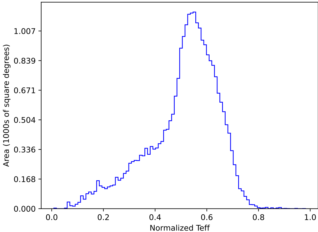
too_elab_r256_d3_ugrizy_v3.4_10yrs All sky y band: Normalized Teff
