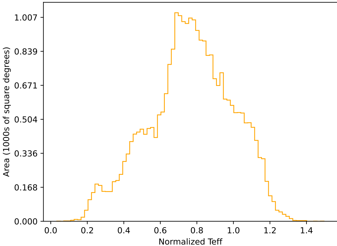
too_elab_r256_d3_ugrizy_v3.4_10yrs All sky r band: Normalized Teff
