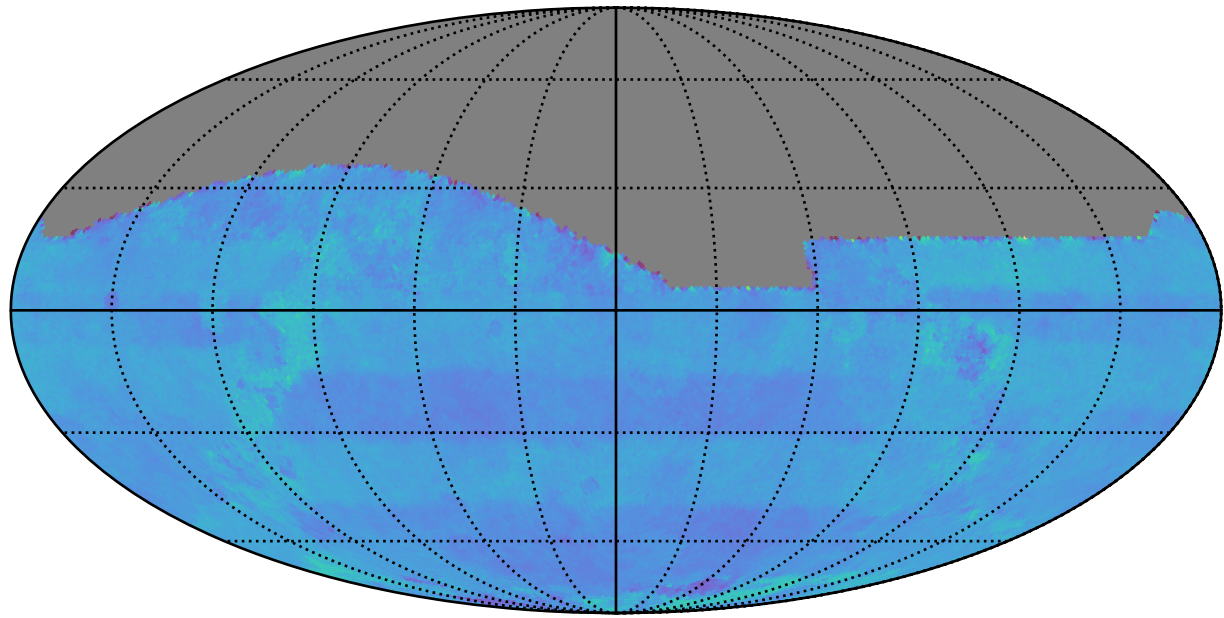
too_elab_r256_d3_ugrizy_v3.4_10yrs All sky: Normalized Proper Motion Uncert @ 24.0
