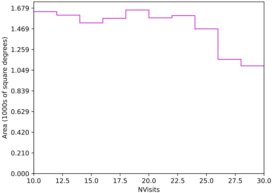
too_elab_r256_d3_ugrizy_v3.4_10yrs Yr 3-4 z band: NVisits
