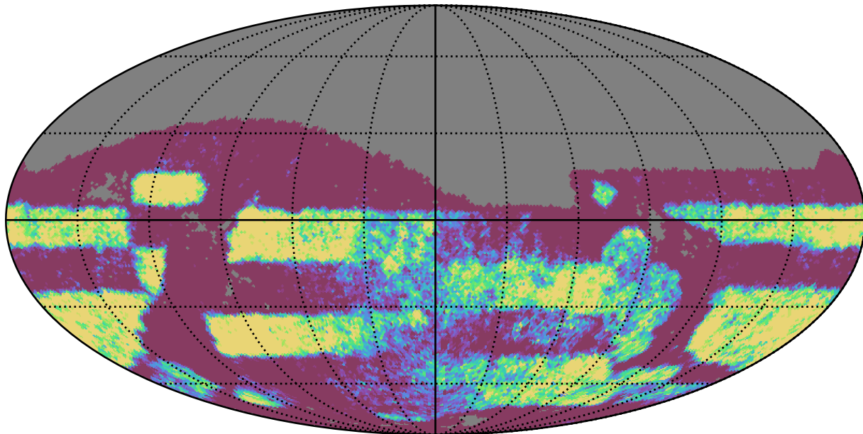
too_elab_r256_d3_ugrizy_v3.4_10yrs Yr 3-4 r band: NVisits
