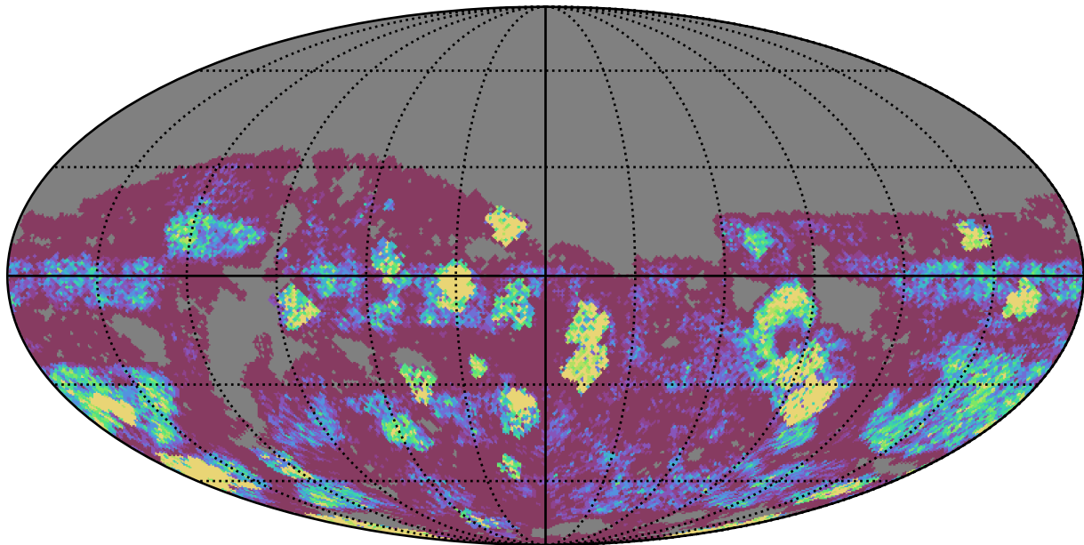
too_elab_r256_d3_ugrizy_v3.4_10yrs Yr 3-4 g band: NVisits
