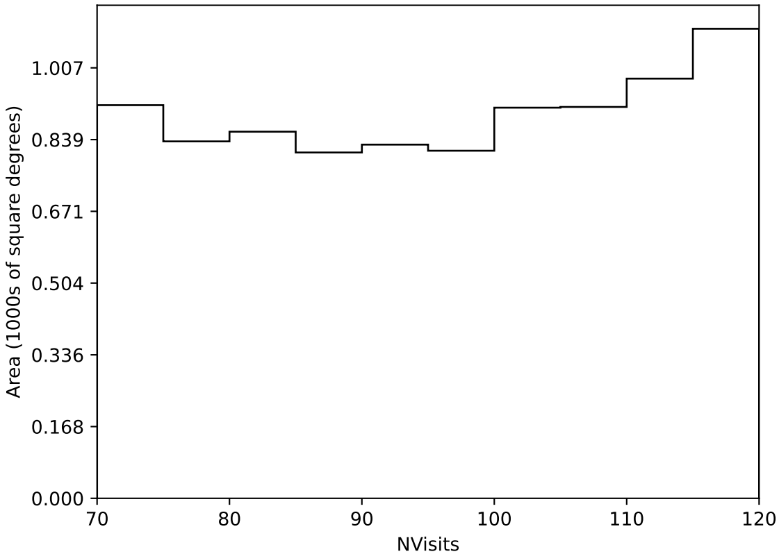
too_elab_r256_d3_ugrizy_v3.4_10yrs Yr 3-4 all bands: NVisits
