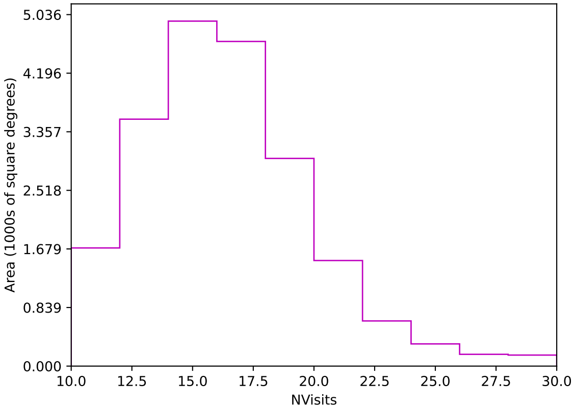
too_elab_r256_d3_ugrizy_v3.4_10yrs Yr 1 z band: NVisits
