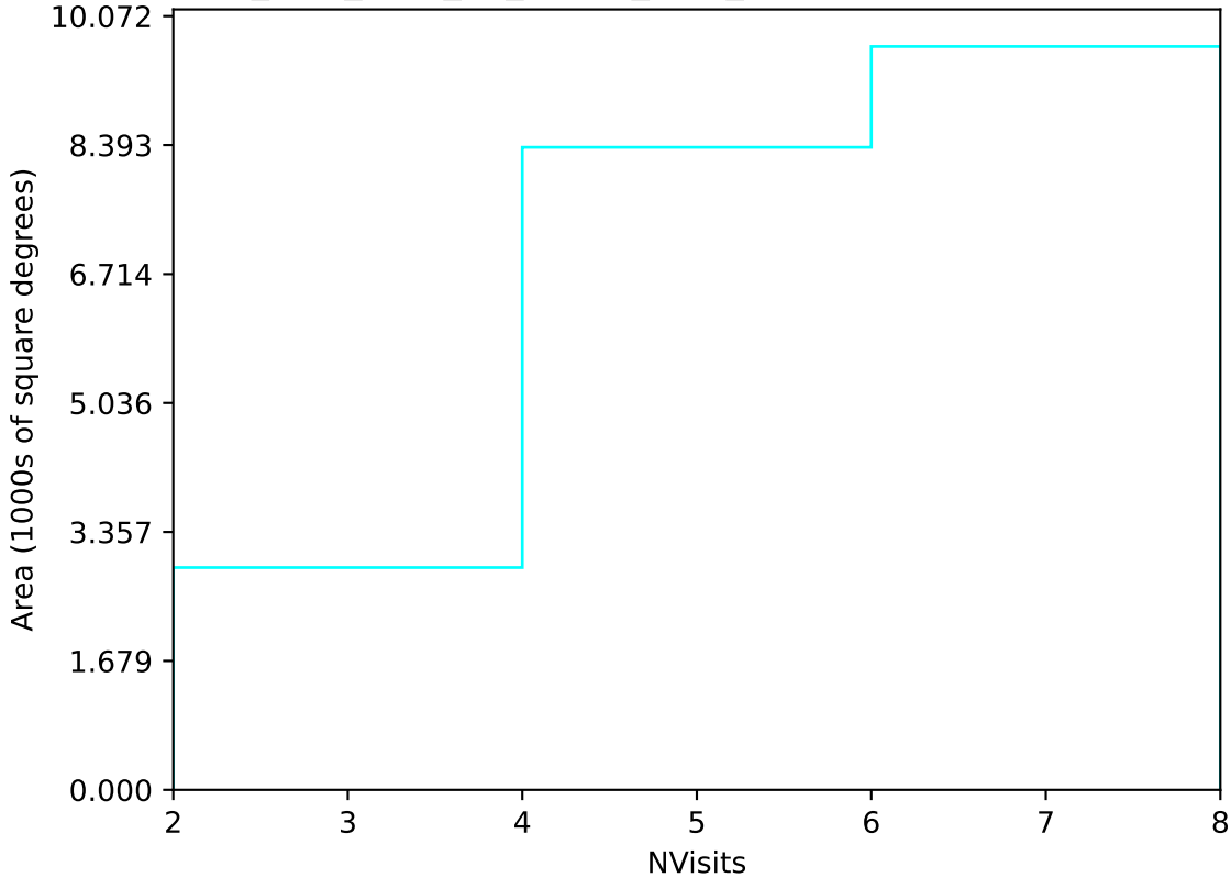
too_elab_r256_d3_ugrizy_v3.4_10yrs Yr 1 u band: NVisits
