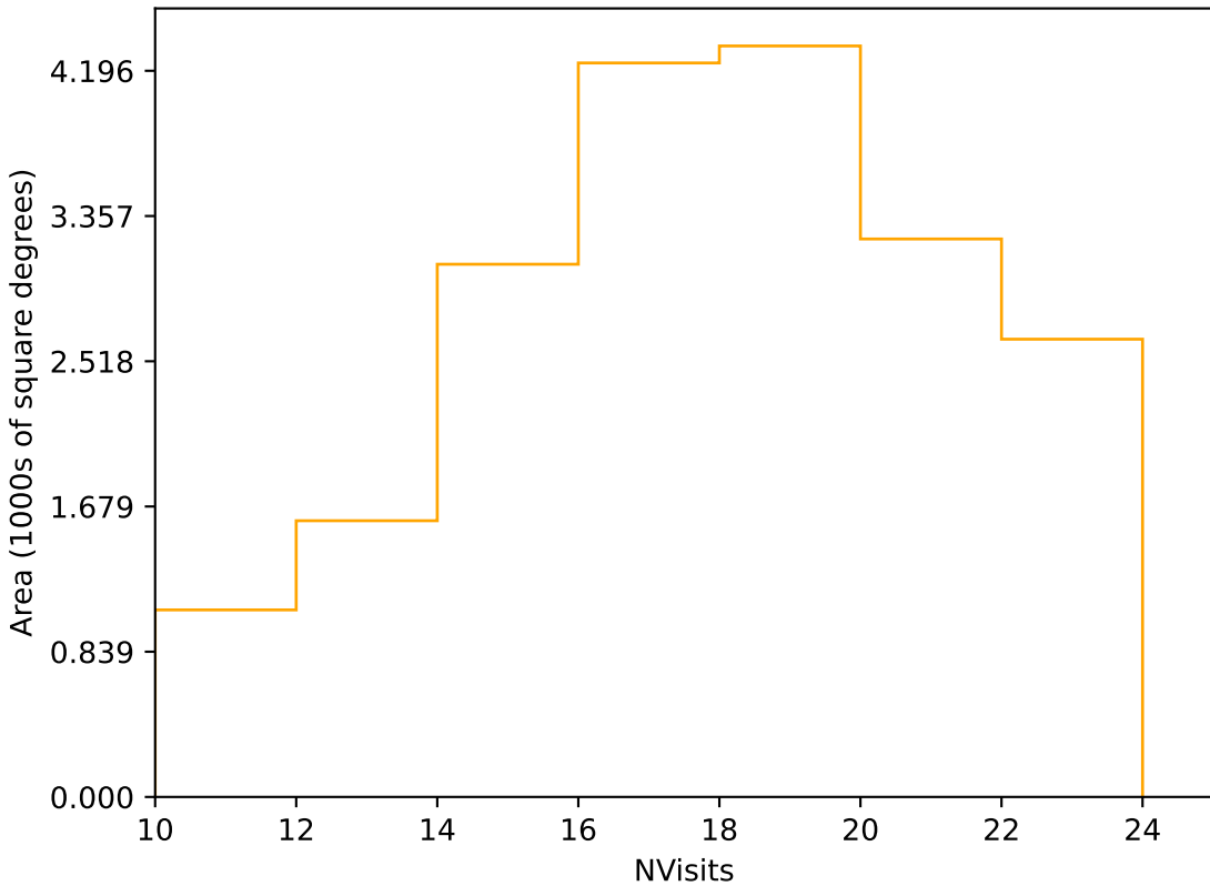
too_elab_r256_d3_ugrizy_v3.4_10yrs Yr 1 r band: NVisits
