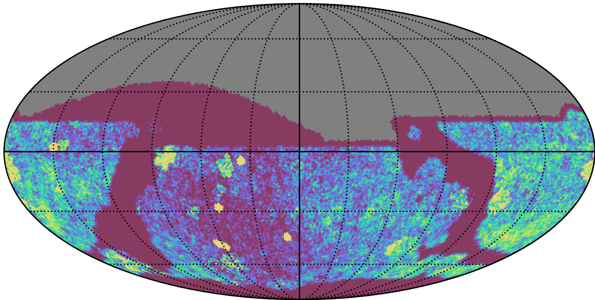
too_elab_r256_d3_ugrizy_v3.4_10yrs Yr 1 all bands: NVisits
