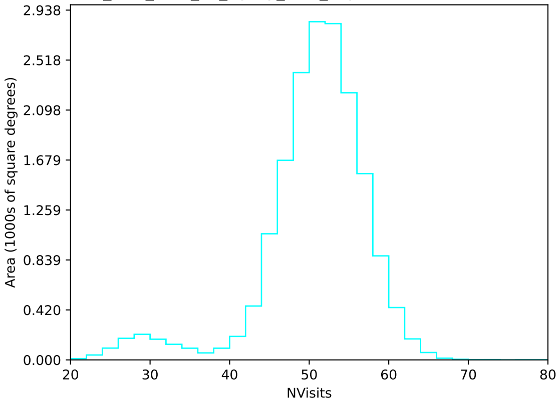
too_elab_r256_d3_ugrizy_v3.4_10yrs WFD u band: NVisits
