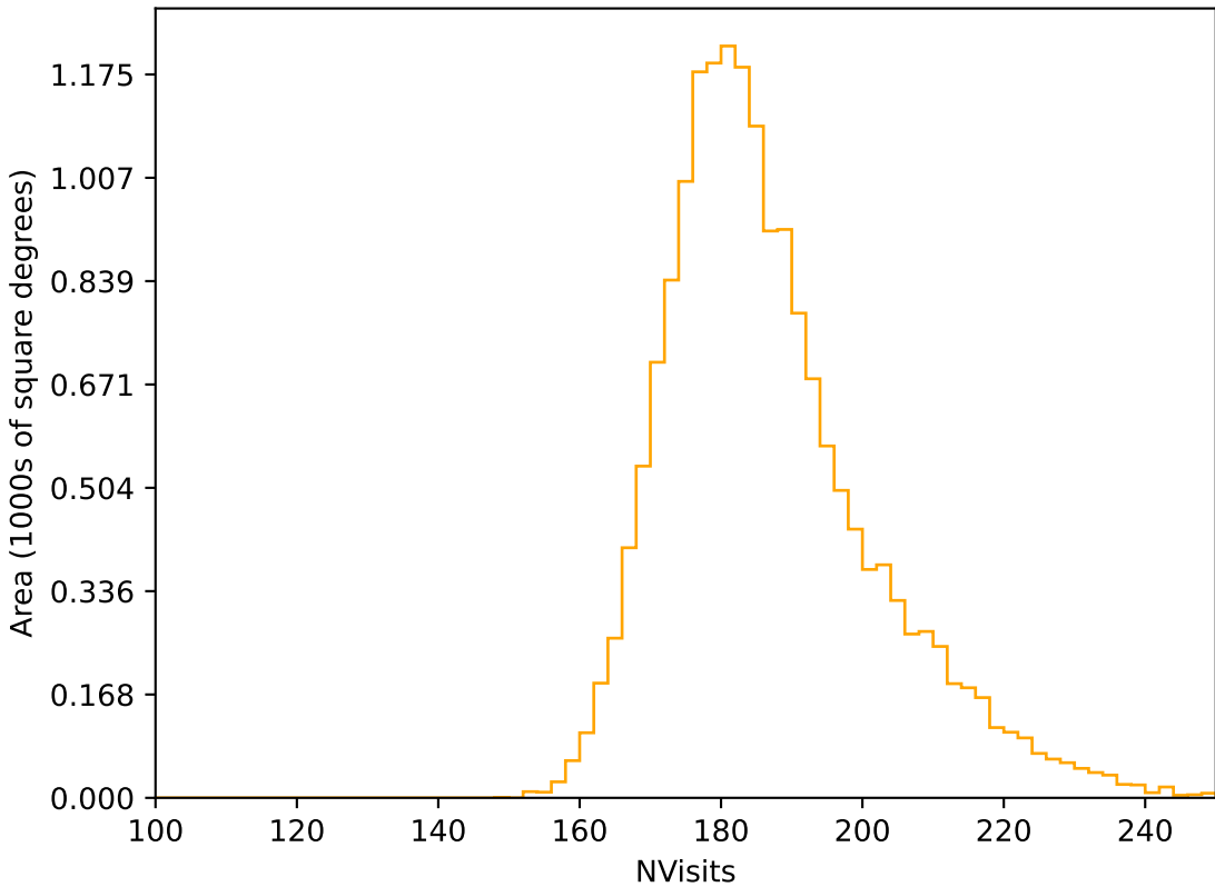
too_elab_r256_d3_ugrizy_v3.4_10yrs WFD r band: NVisits
