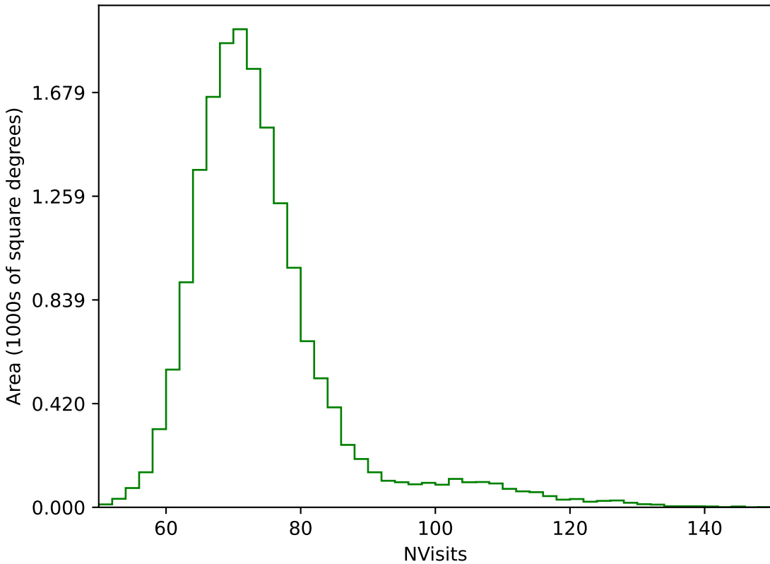
too_elab_r256_d3_ugrizy_v3.4_10yrs WFD g band: NVisits
