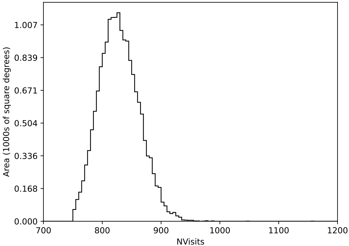
too_elab_r256_d3_ugrizy_v3.4_10yrs WFD all bands: NVisits
