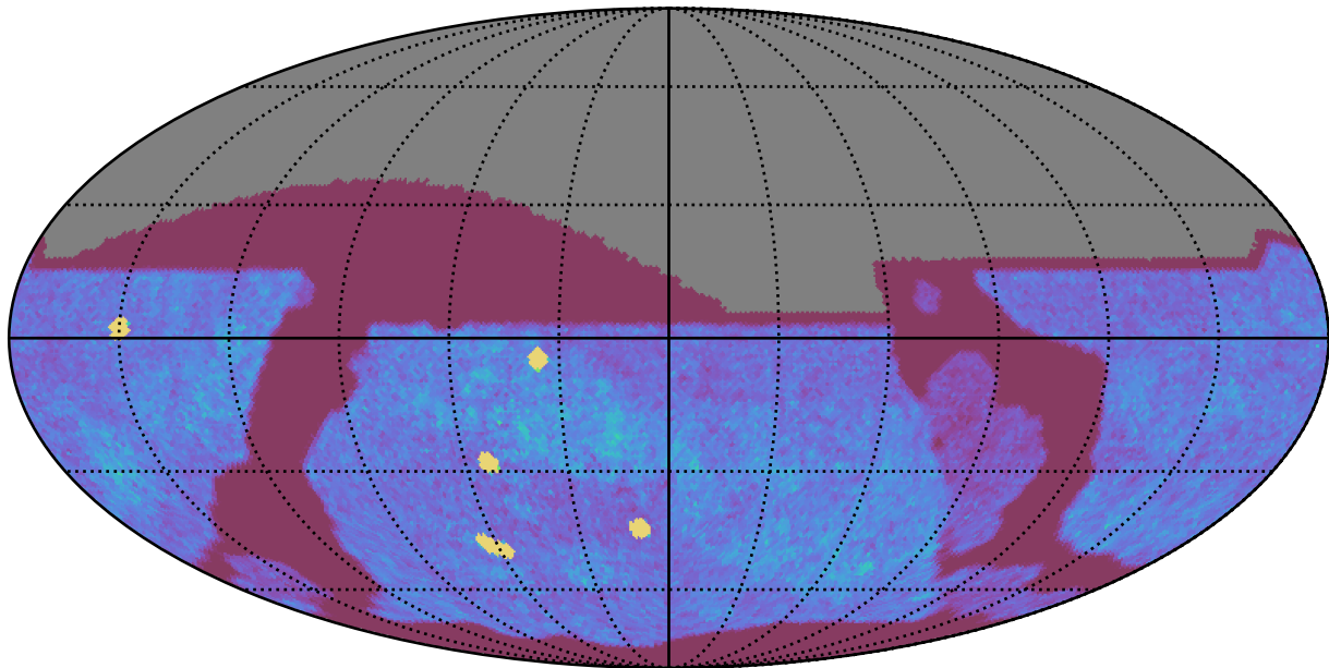
too_elab_r256_d3_ugrizy_v3.4_10yrs All sky z band: NVisits
