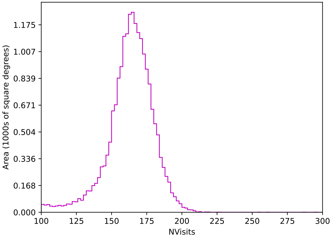
too_elab_r256_d3_ugrizy_v3.4_10yrs All sky z band: NVisits
