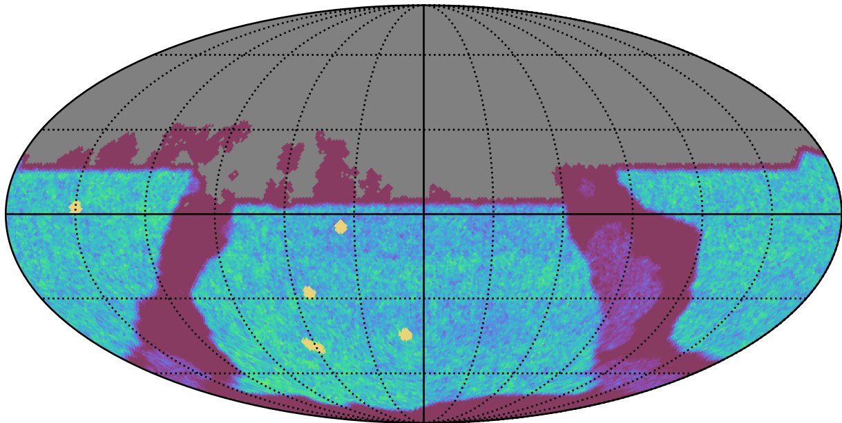
too_elab_r256_d3_ugrizy_v3.4_10yrs All sky u band: NVisits
