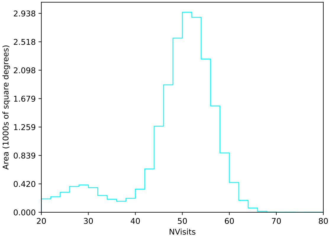
too_elab_r256_d3_ugrizy_v3.4_10yrs All sky u band: NVisits
