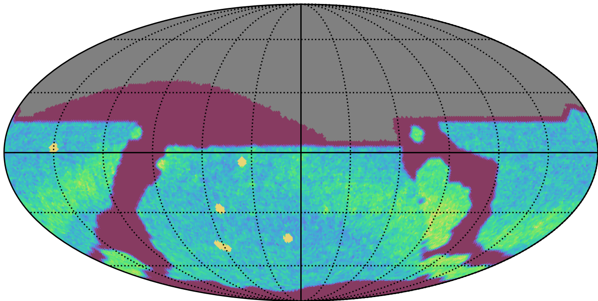
too_elab_r256_d3_ugrizy_v3.4_10yrs All sky r band: NVisits
