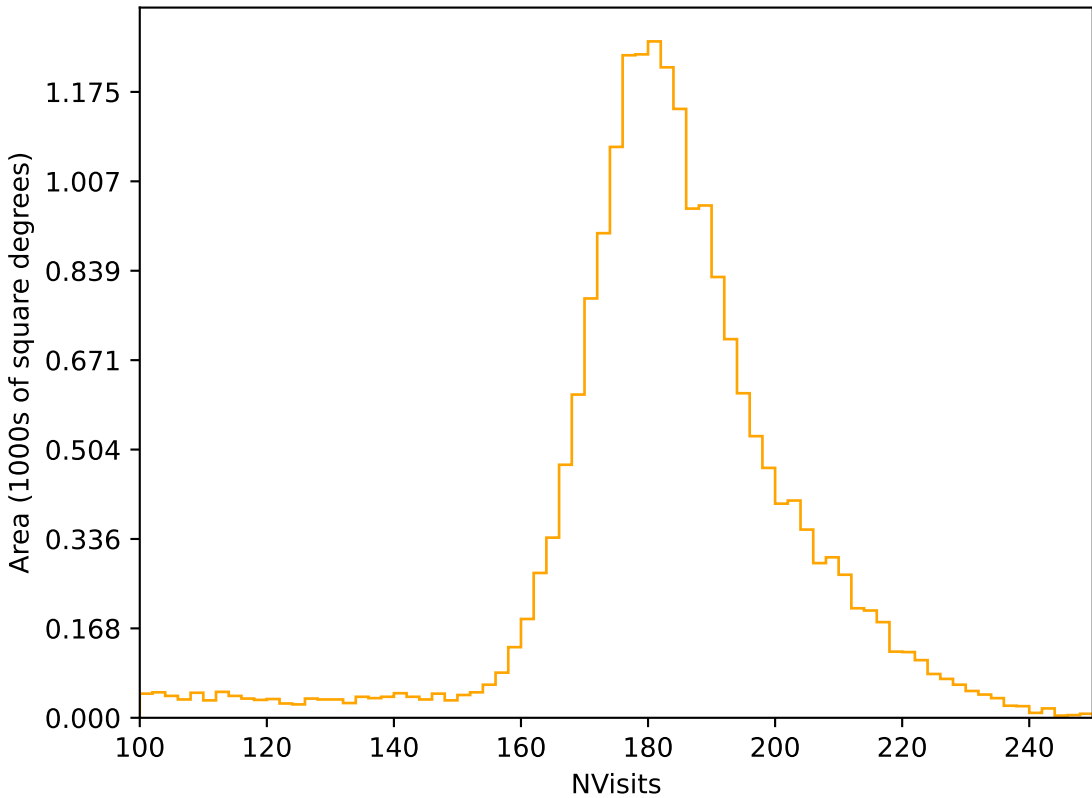
too_elab_r256_d3_ugrizy_v3.4_10yrs All sky r band: NVisits
