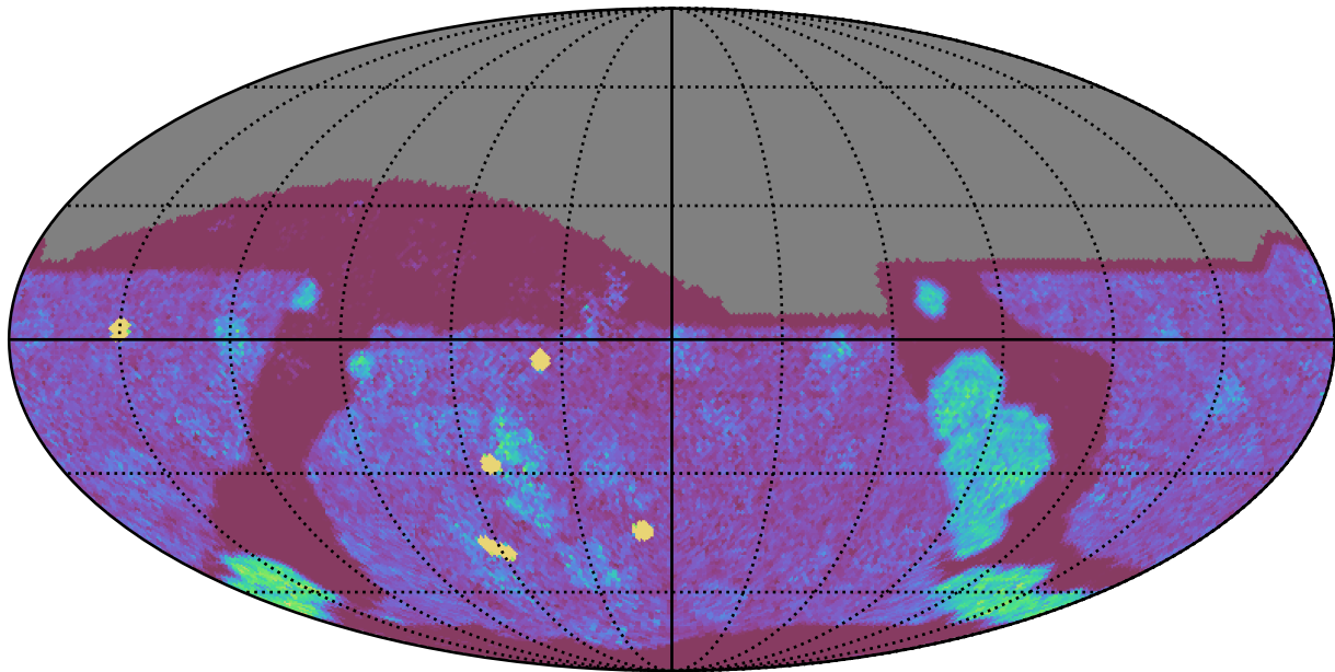
too_elab_r256_d3_ugrizy_v3.4_10yrs All sky g band: NVisits
