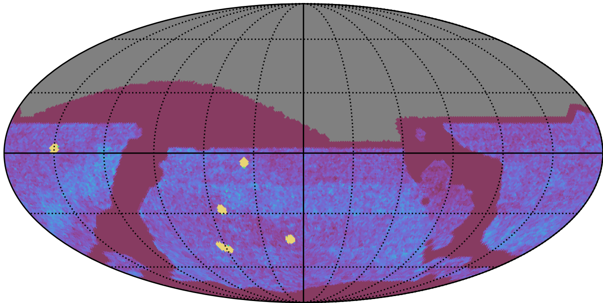
too_elab_r256_d3_ugrizy_v3.4_10yrs All sky all bands: NVisits
