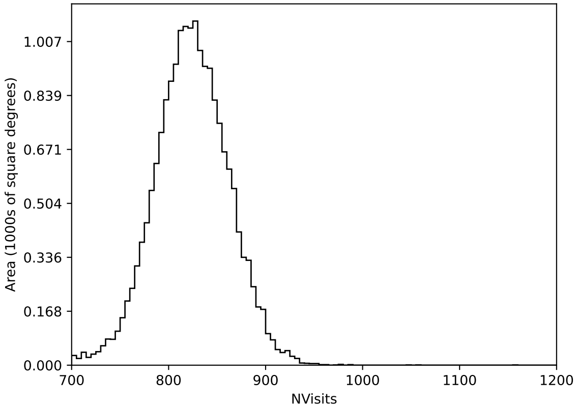
too_elab_r256_d3_ugrizy_v3.4_10yrs All sky all bands: NVisits
