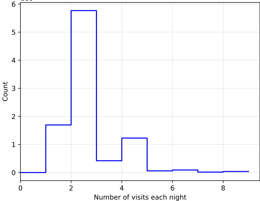
too_elab_r256_d3_ugrizy_v3.4_10yrs All sky: NVisitsPerNight 1e6
