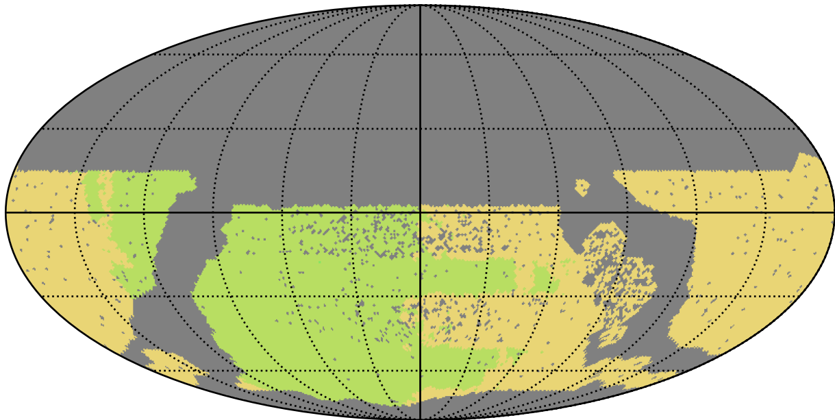
too_elab_r256_d3_ugrizy_v3.4_10yrs WFD all bands: NSeasons
