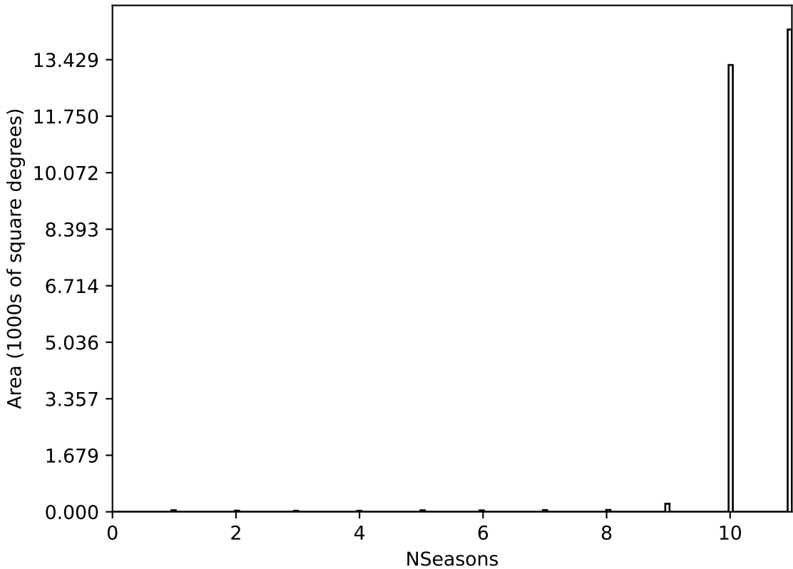
too_elab_r256_d3_ugrizy_v3.4_10yrs All sky all bands: NSeasons
