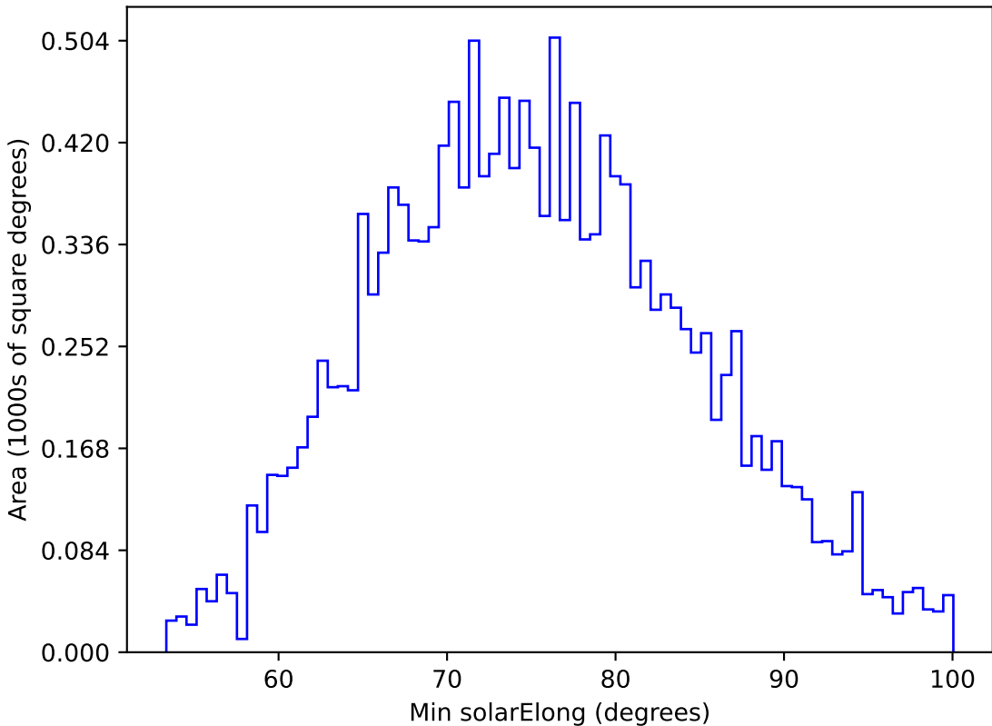
too_elab_r256_d3_ugrizy_v3.4_10yrs WFD u band: Min solarElong
