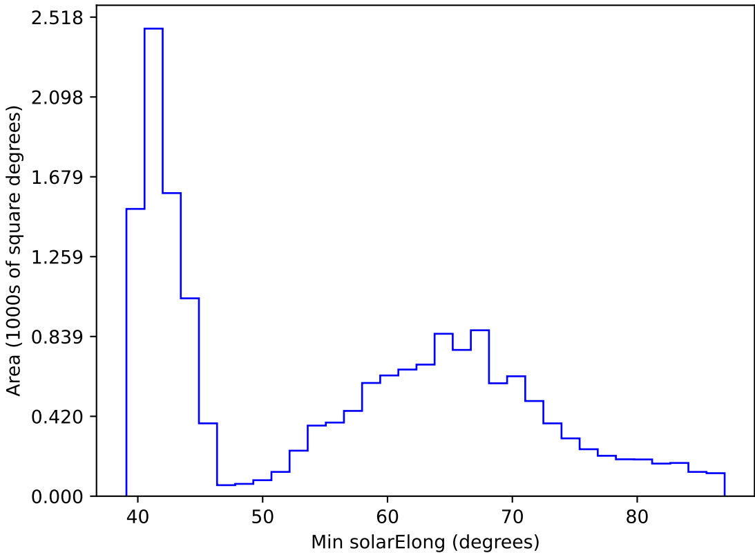
too_elab_r256_d3_ugrizy_v3.4_10yrs WFD r band: Min solarElong
