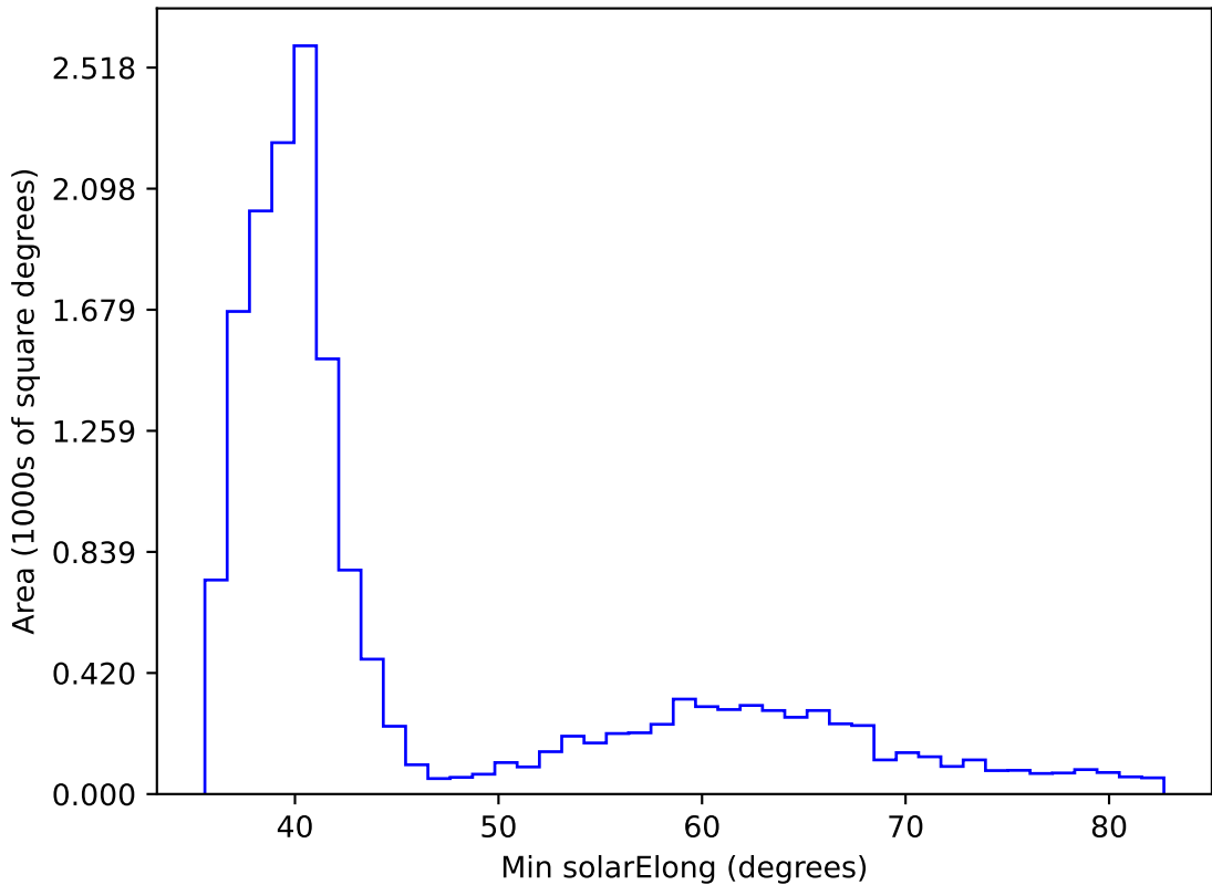
too_elab_r256_d3_ugrizy_v3.4_10yrs WFD all bands: Min solarElong
