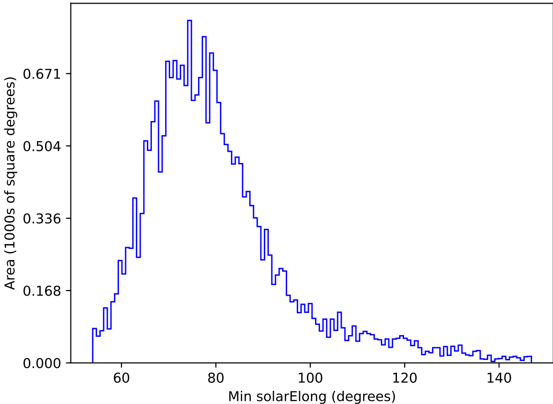
too_elab_r256_d3_ugrizy_v3.4_10yrs All sky u band: Min solarElong
