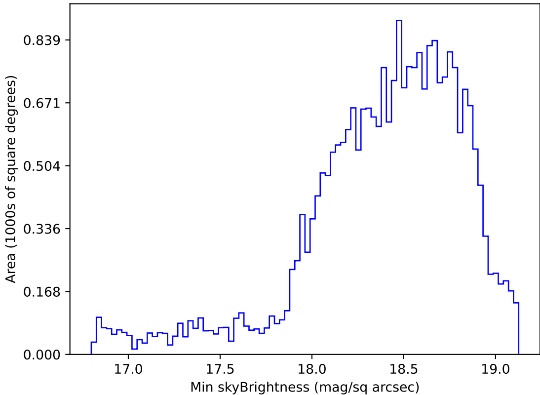
too_elab_r256_d3_ugrizy_v3.4_10yrs Yr 1 z band: Min skyBrightness
