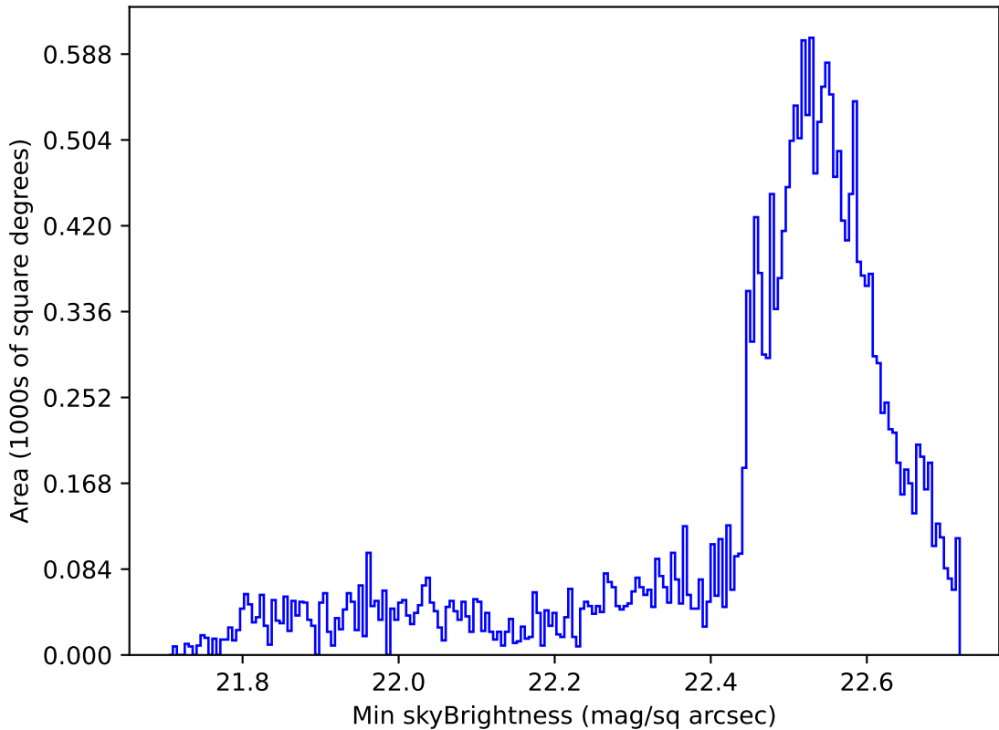
too_elab_r256_d3_ugrizy_v3.4_10yrs Yr 1 u band: Min skyBrightness
