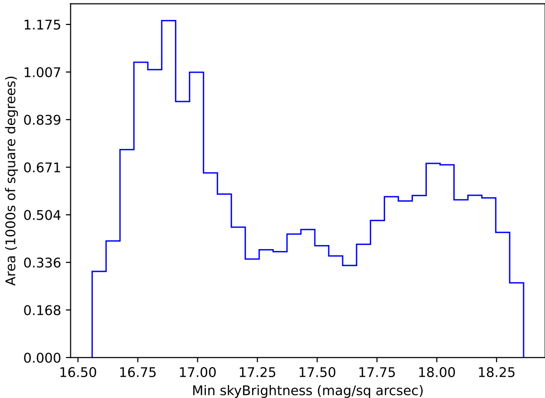
too_elab_r256_d3_ugrizy_v3.4_10yrs WFD z band: Min skyBrightness
