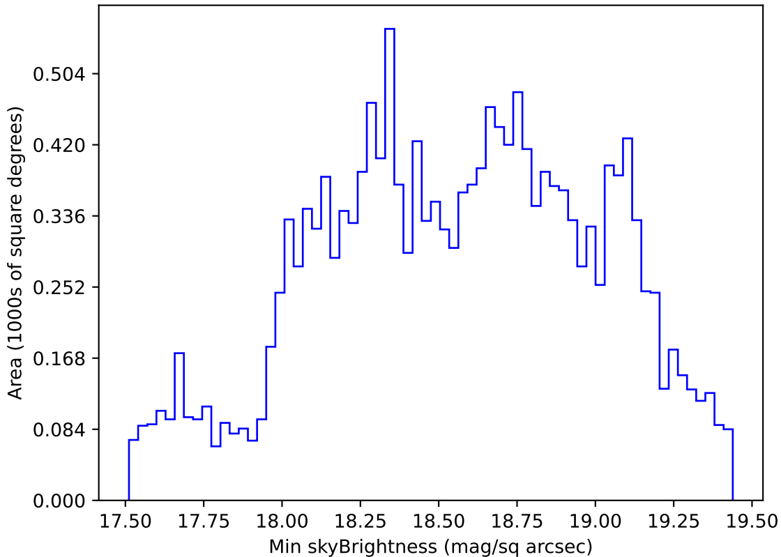
too_elab_r256_d3_ugrizy_v3.4_10yrs WFD r band: Min skyBrightness
