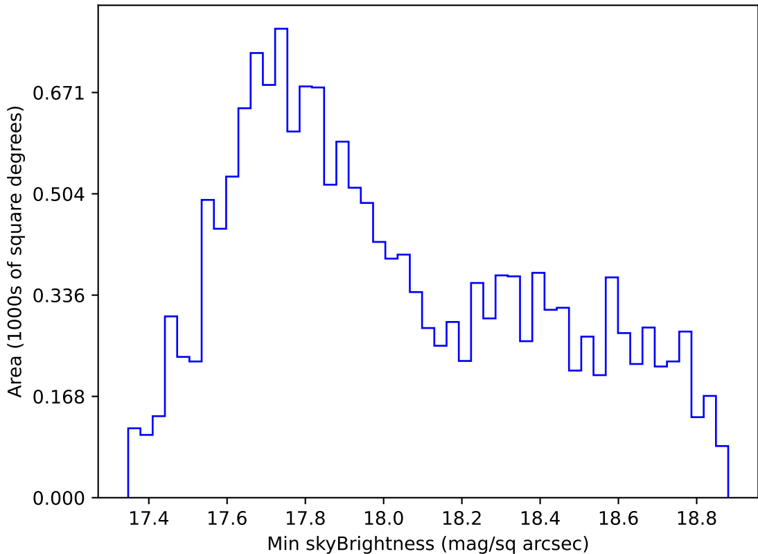
too_elab_r256_d3_ugrizy_v3.4_10yrs WFD i band: Min skyBrightness
