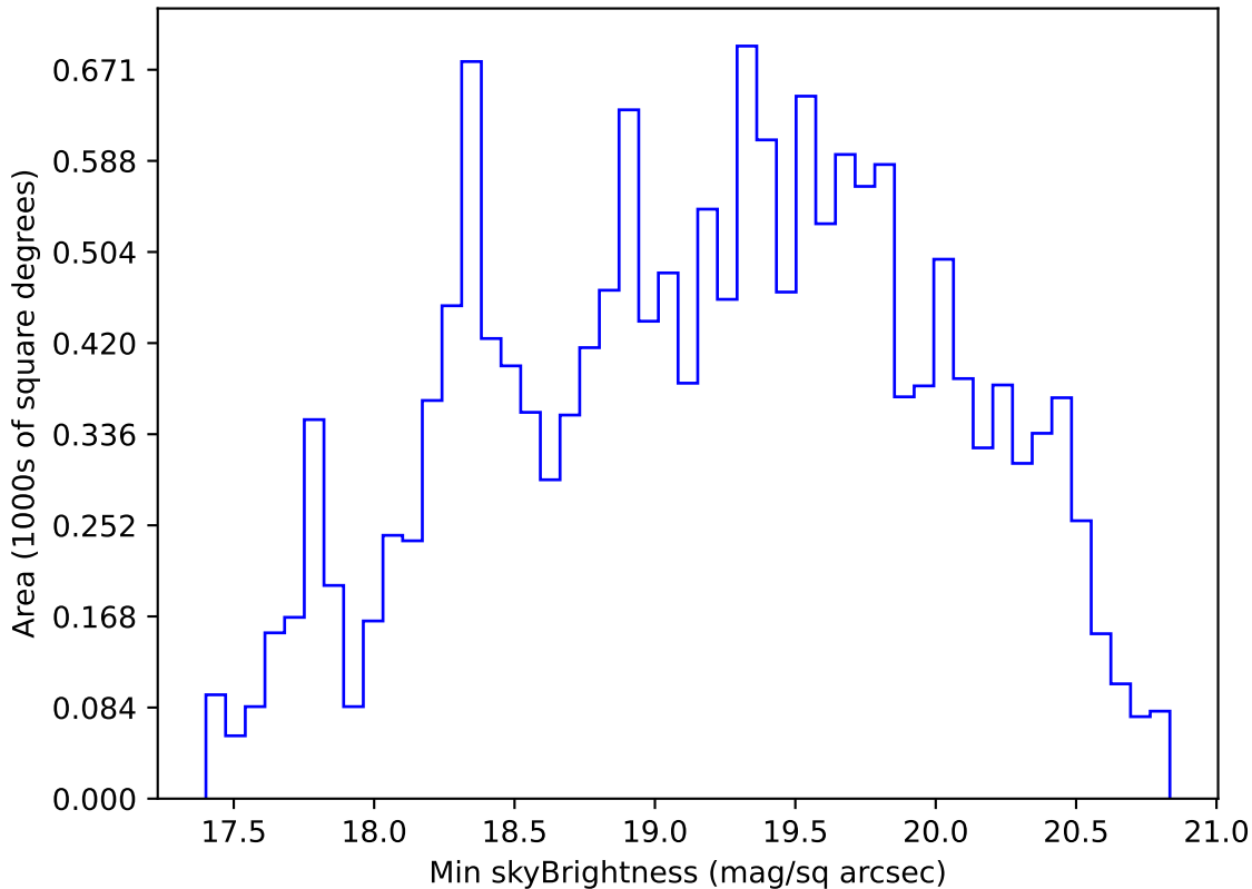
too_elab_r256_d3_ugrizy_v3.4_10yrs WFD g band: Min skyBrightness
