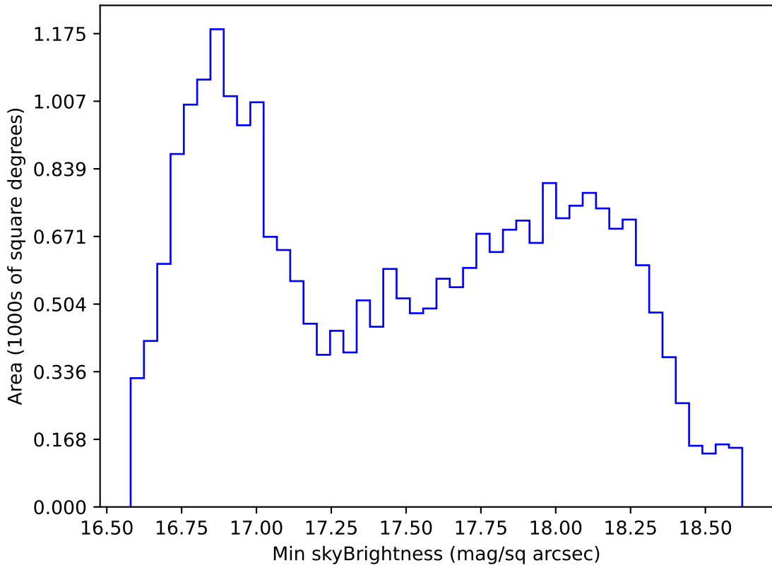
too_elab_r256_d3_ugrizy_v3.4_10yrs All sky z band: Min skyBrightness
