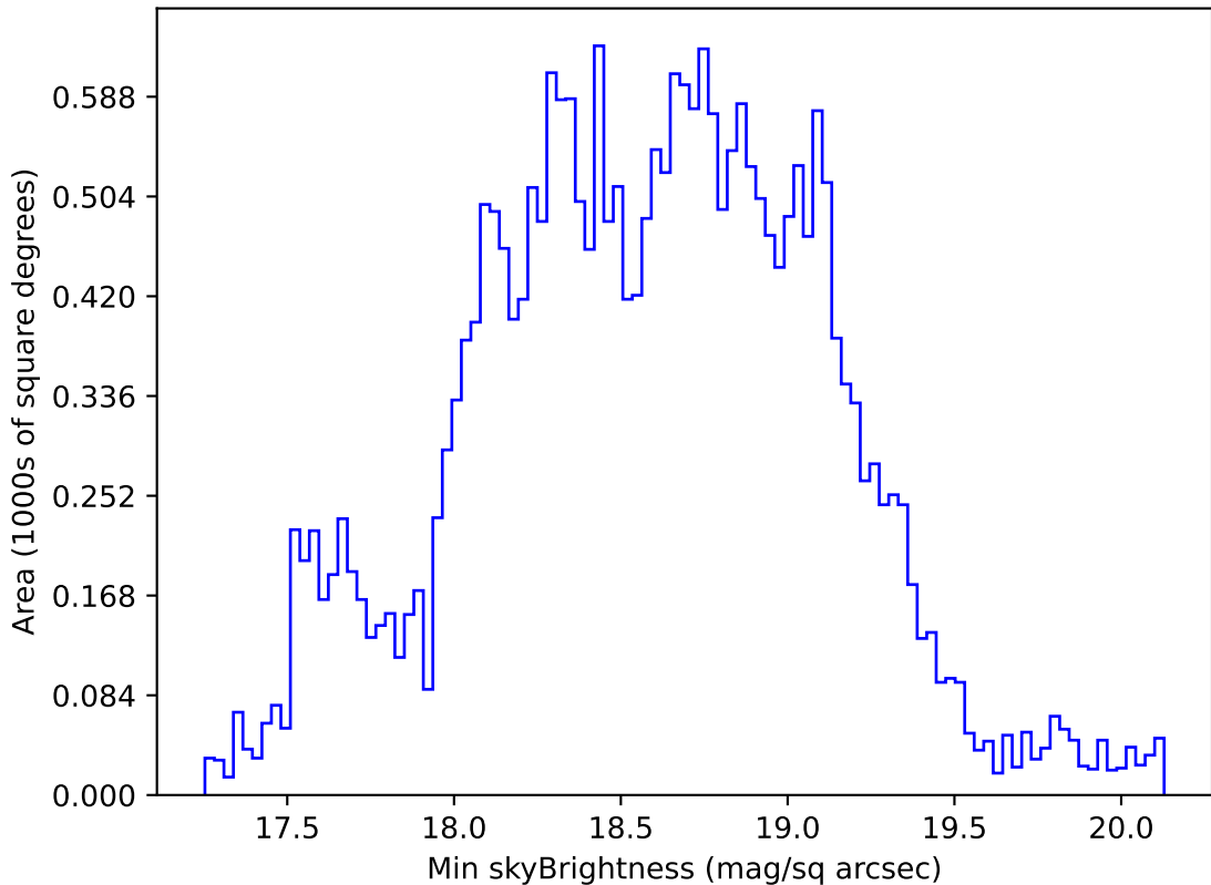
too_elab_r256_d3_ugrizy_v3.4_10yrs All sky r band: Min skyBrightness
