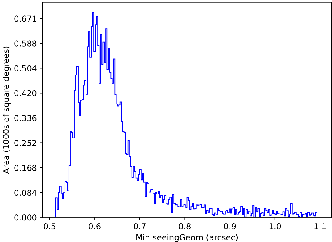
too_elab_r256_d3_ugrizy_v3.4_10yrs Yr 1 r band: Min seeingGeom
