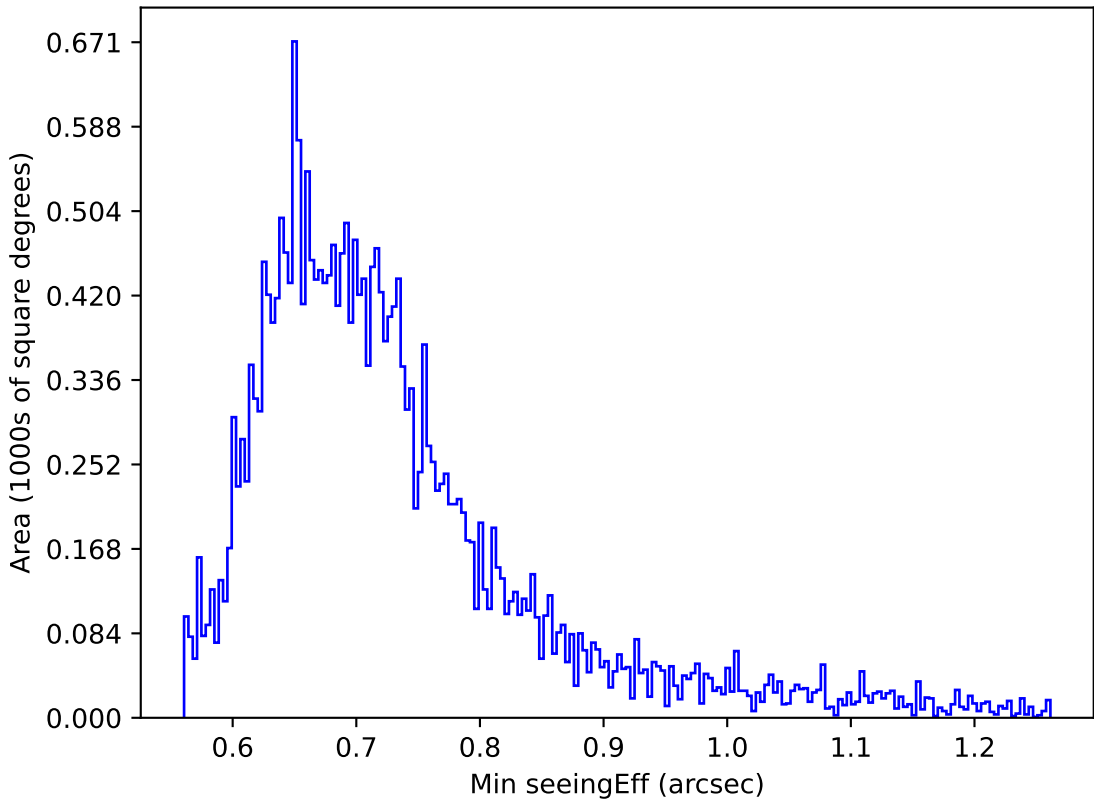
too_elab_r256_d3_ugrizy_v3.4_10yrs Yr 1 z band: Min seeingEff
