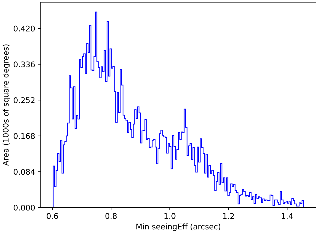
too_elab_r256_d3_ugrizy_v3.4_10yrs Yr 1 u band: Min seeingEff
