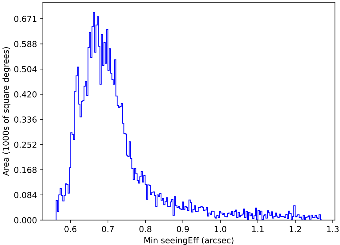
too_elab_r256_d3_ugrizy_v3.4_10yrs Yr 1 r band: Min seeingEff
