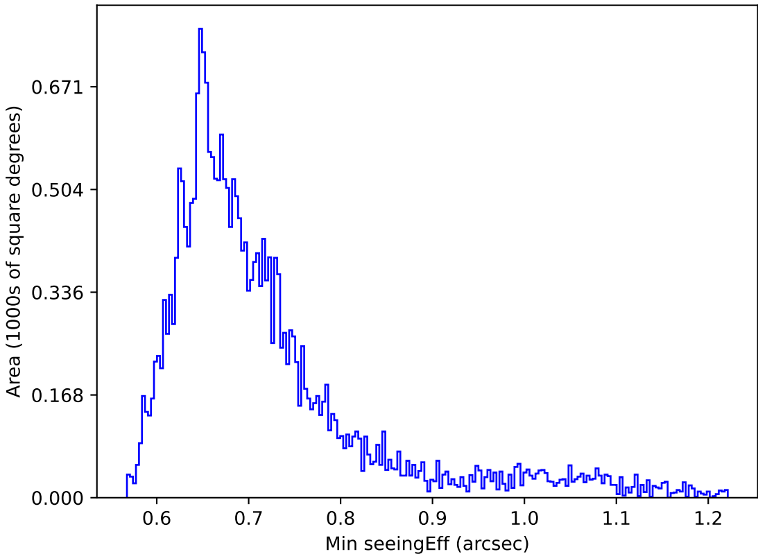
too_elab_r256_d3_ugrizy_v3.4_10yrs Yr 1 i band: Min seeingEff
